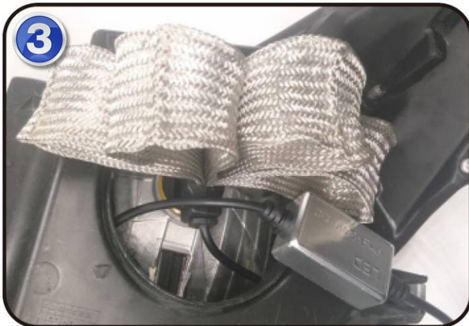
3 SPREAD HEATSINK OUT AS FAR AS POSSIBLE. SECURE LED DRIVER BOX.
